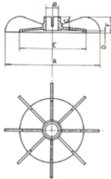
MOTOR COOLING FANS V series
